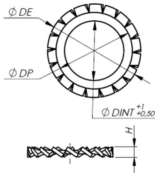
Technical Illustration
